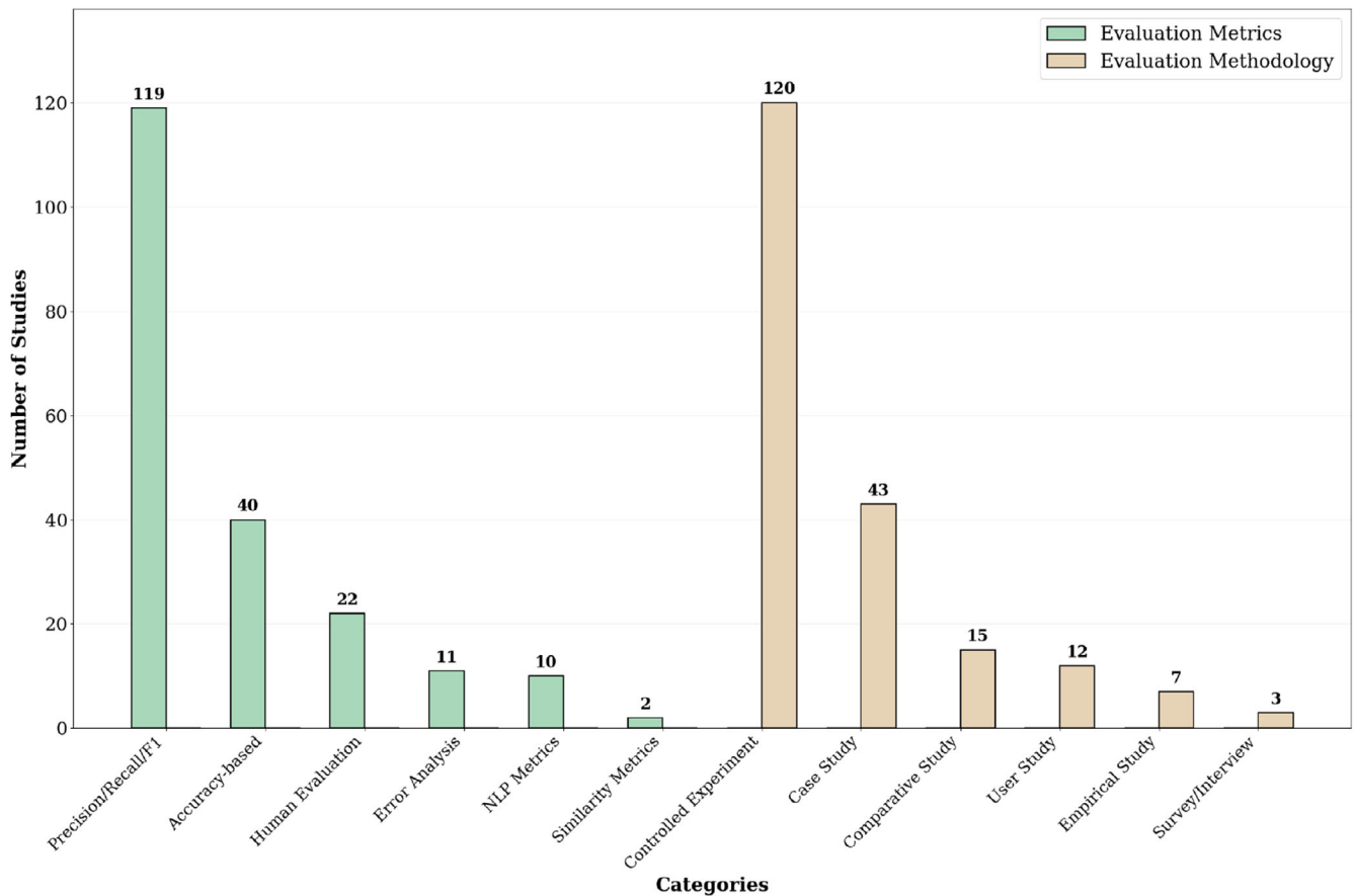
FIGURE 12 | Distribution of evaluation metrics and methodology ( N = 238 ).
